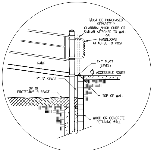
SUGGESTED ELEVATED RAMP EXIT INSTALLATION RAMP ELEVATION TO BE 8" ABOVE FINISH GRADE.
