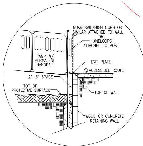
SUGGESTED ELEVATED RAMP EXIT INSTALLATION RAMP ELEVATION TO BE 24" ABOVE FINISH GRADE.
